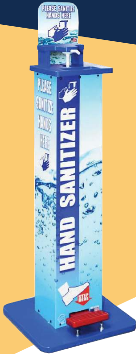
STANDARD MODEL
