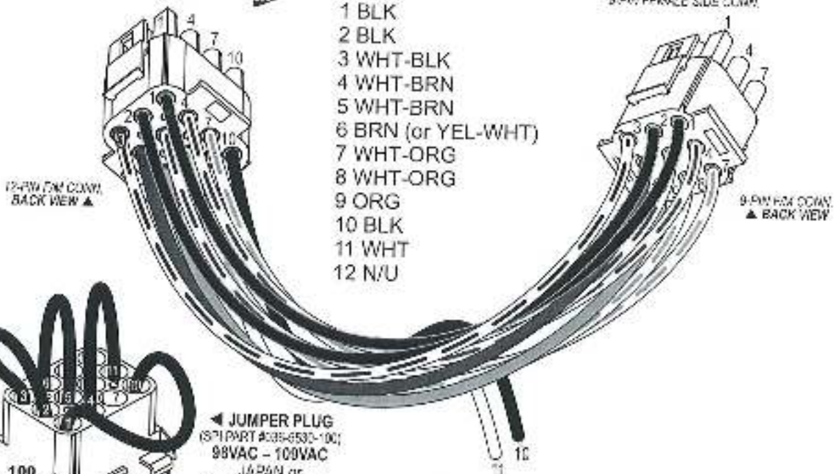
9-PIN MALE SIDE TO TRANSFORMER 9-PIN FEMALE SIDE DOWN
